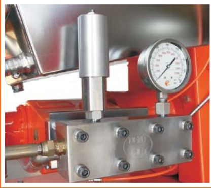
Stainless steel pump-head. Integrated feed pump.
